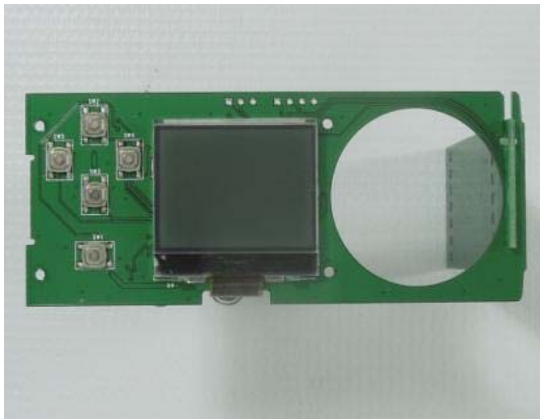
Fig. 2a PCB (Front view)
